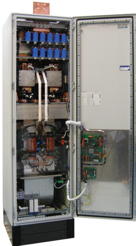
POWER STATION pe5110, front view
