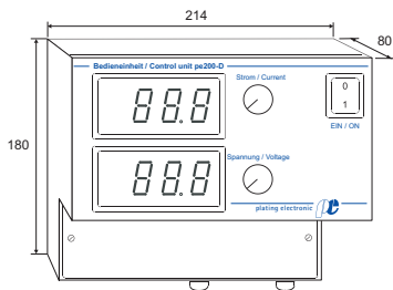
Control unit pe200-D standard, dimensions
